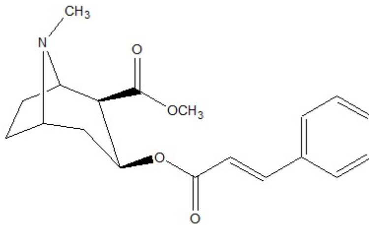
(E)-form Cinnamoylcocaine
